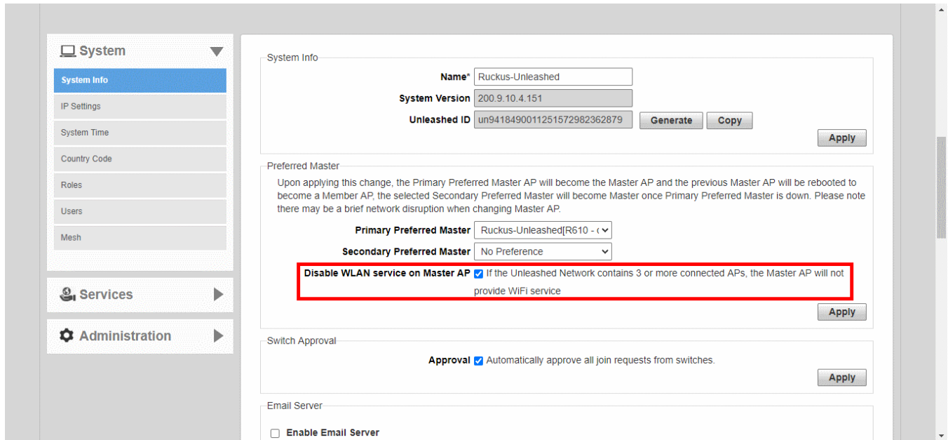
FIGURE 226 Disabling Master AP WLAN service
