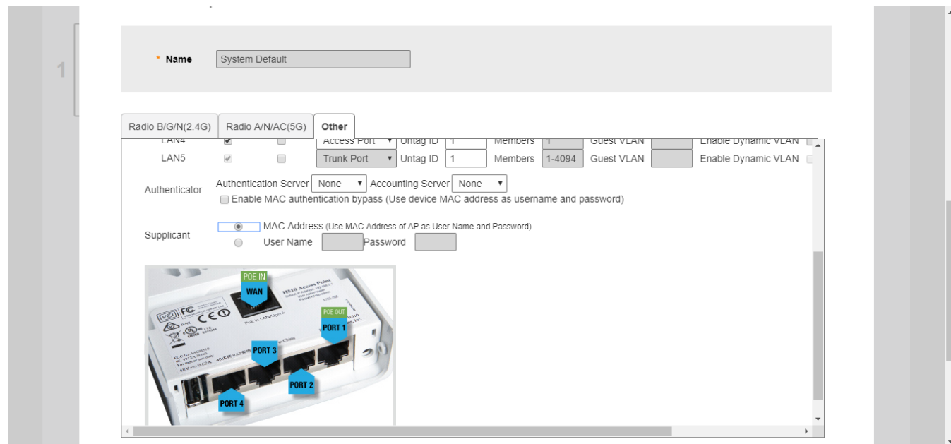
FIGURE 177 H510 Authenticator and Supplicant settings
