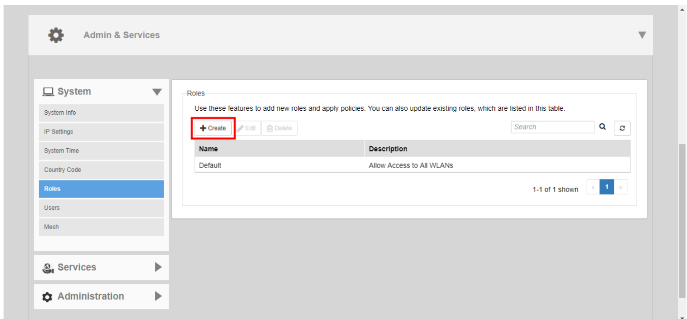
FIGURE 244 Roles
