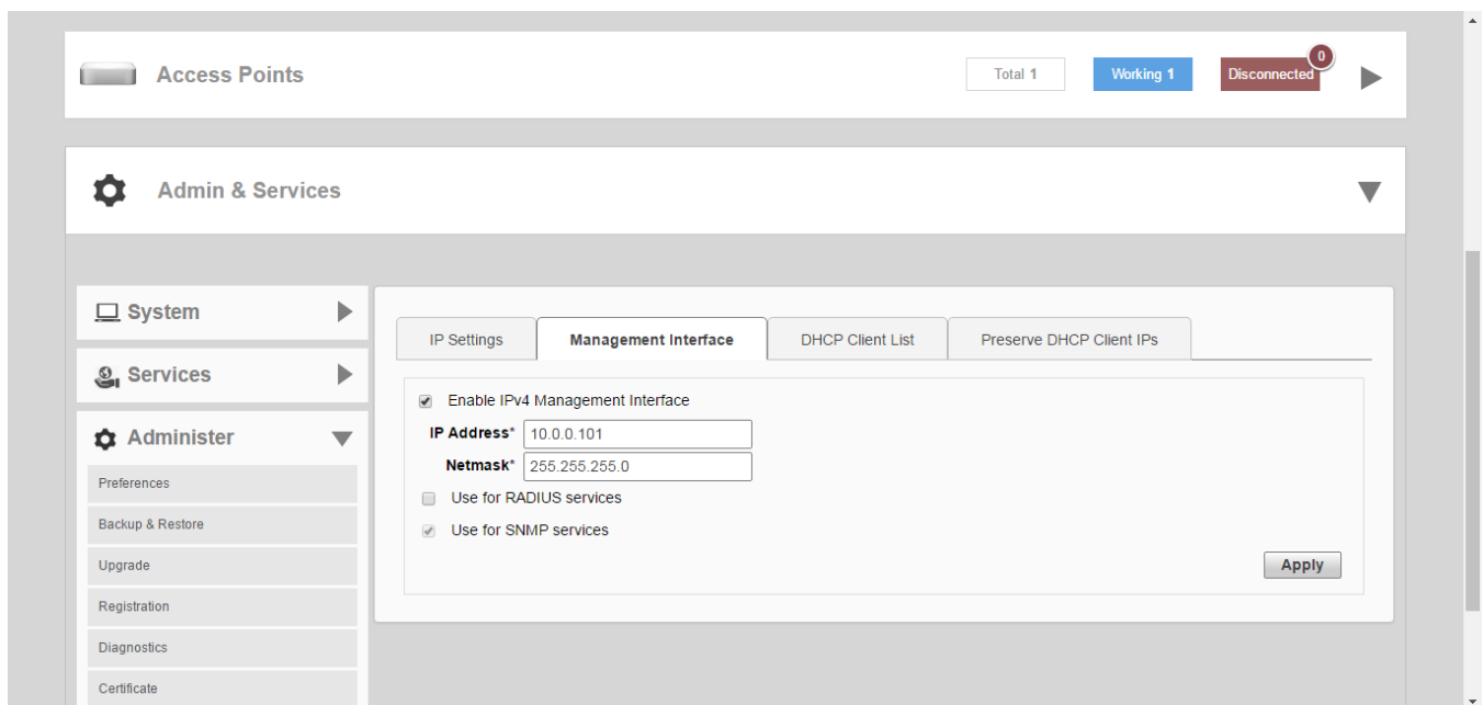
FIGURE 240 Management Interface
