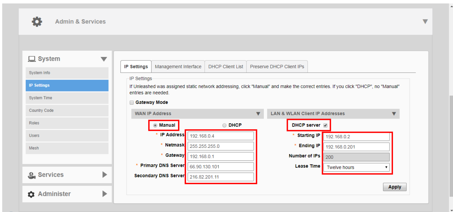
FIGURE 236 DHCP Server configuration
