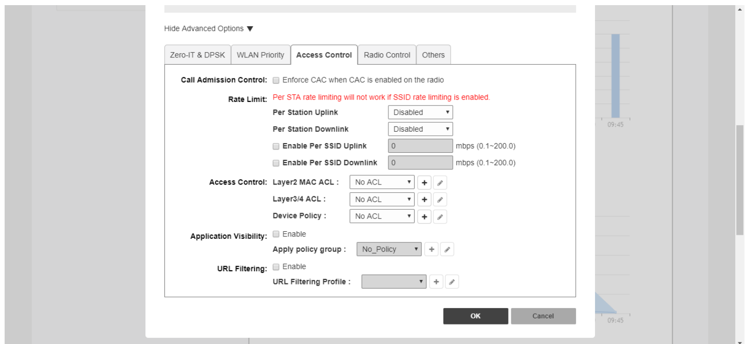
FIGURE 132 Advanced WLAN settings - Access Control configuration
