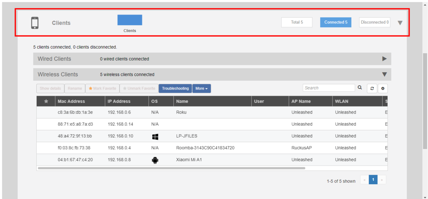
FIGURE 49 Clients Component
