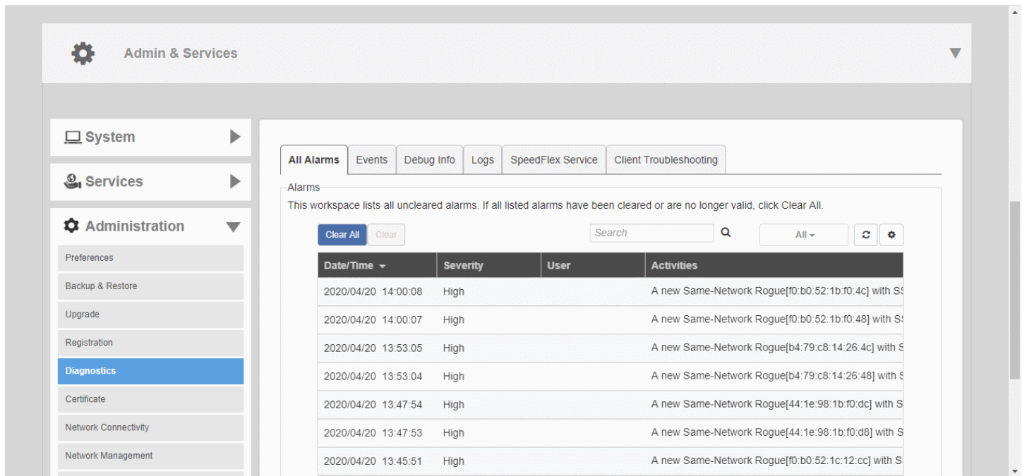
FIGURE 325 Diagnostics
