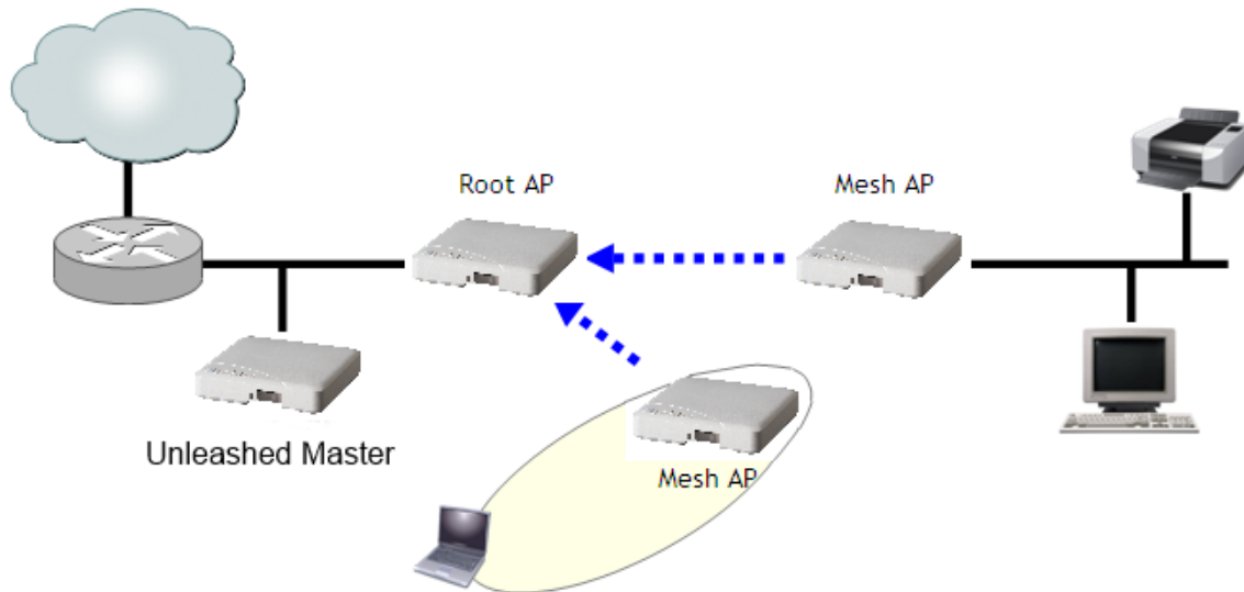
FIGURE 250 Mesh - wireless bridge topology
