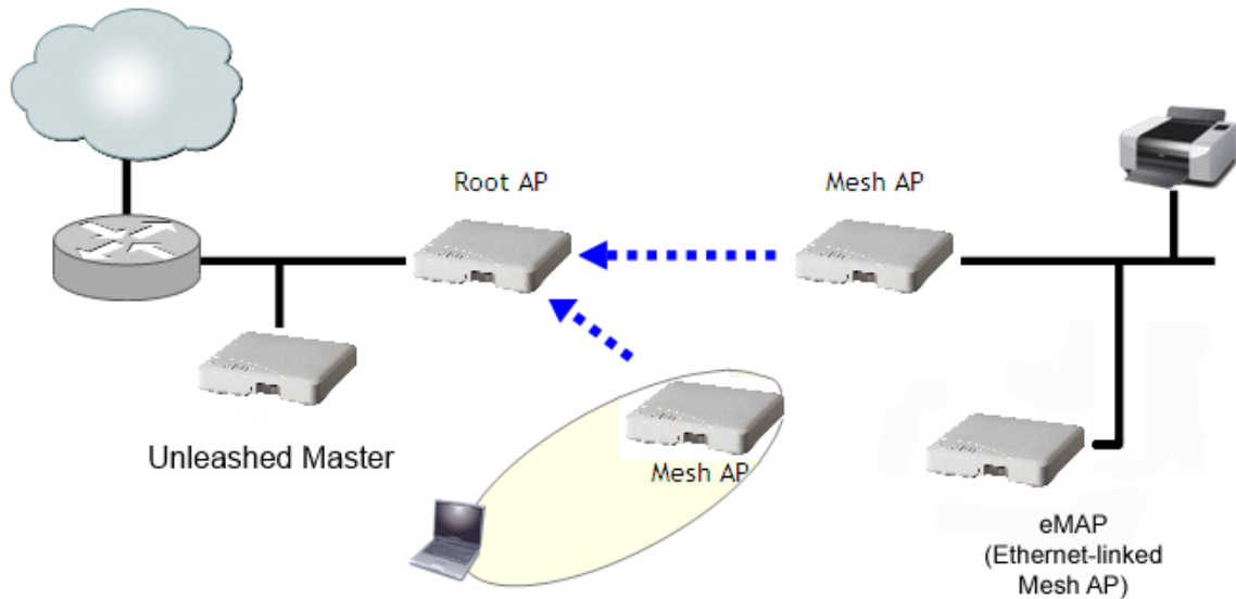
FIGURE 251 eMAP - Hybrid Mesh topology
