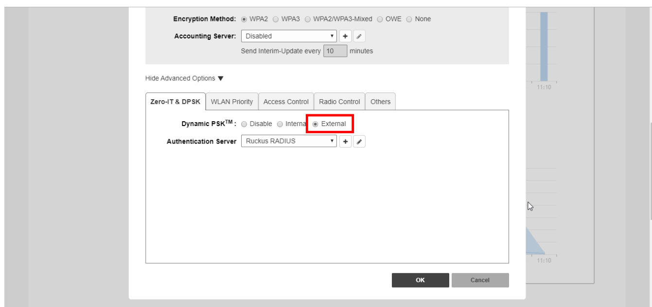
FIGURE 130 External DPSK
