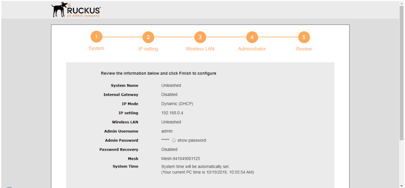
FIGURE 34 Setup Wizard 5
