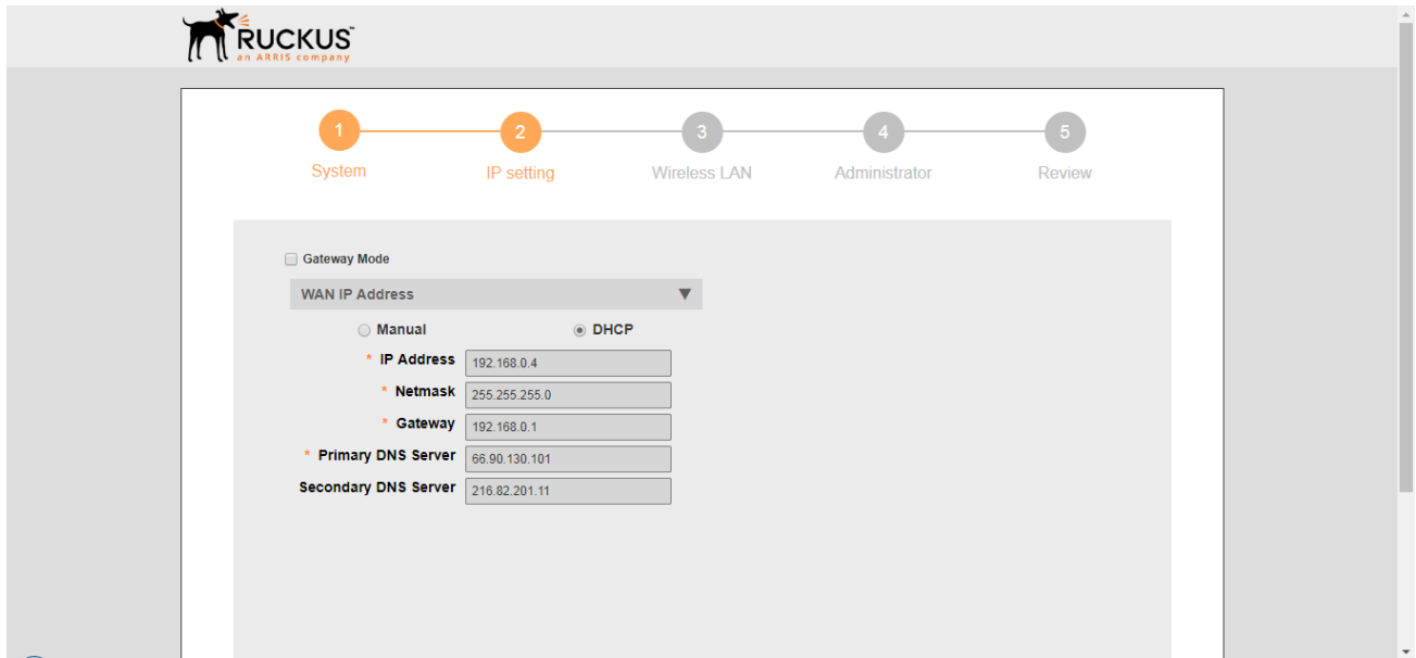
FIGURE 31 Setup Wizard 2
