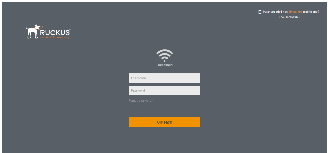
FIGURE 37 Login screen
