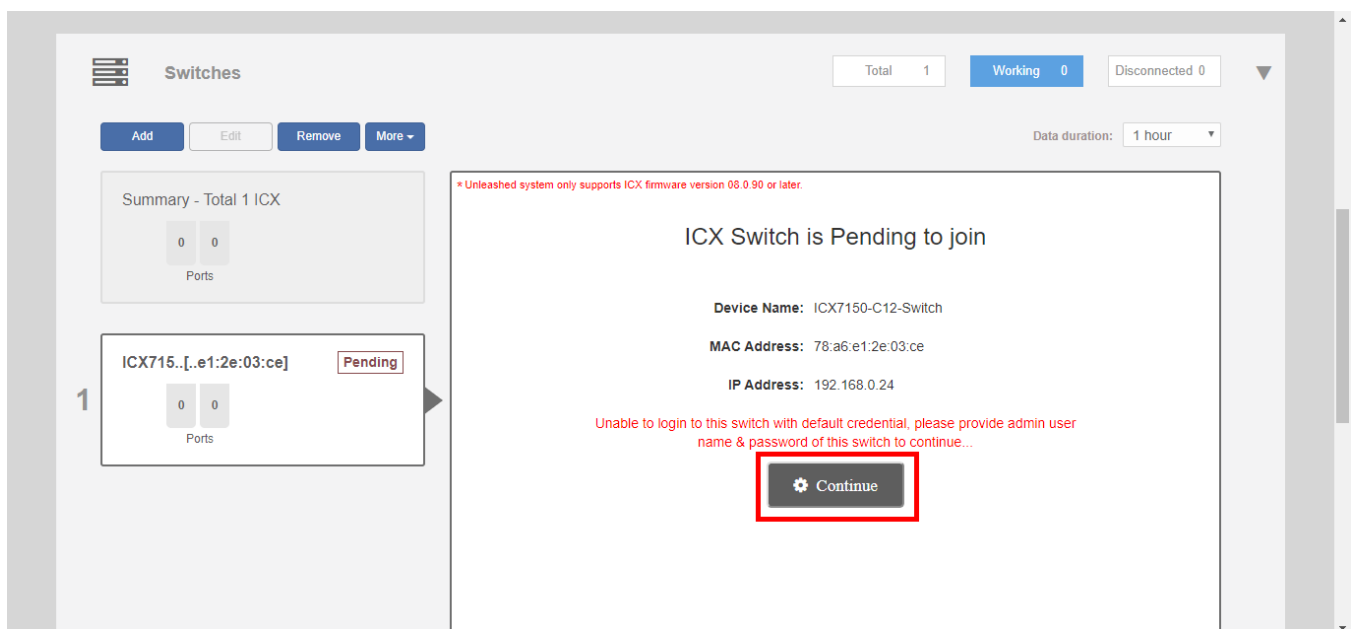
FIGURE 184 Click Continue
