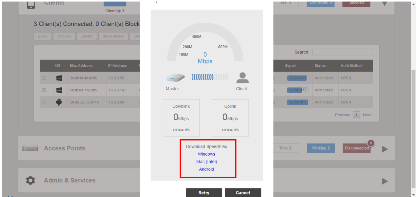
FIGURE 215 Download SpeedFlex
